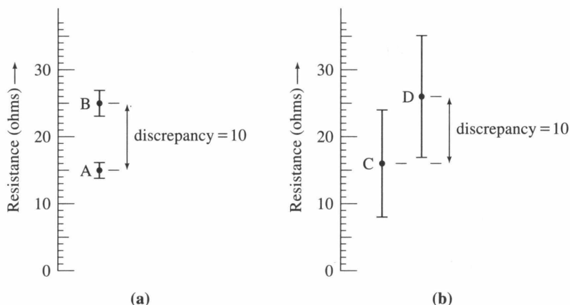
Figure 2.1. (a) Two measurements of the same resistance. Each measurement includes a best estimate, shown by a black dot, and a range of probable values, shown by a vertical error bar. The discrepancy (difference between the two best estimates) is 10 ohms and is significant because it is much larger than the combined uncertainty in the two measurements. Almost certainly, at least one of the experimenters made a mistake. (b) Two different measurements of the same resistance. The discrepancy is again 10 ohms, but in this case it is insignificant because the stated margins of error overlap. There is no reason to doubt either measurement (although they could be criticized for being rather imprecise).
