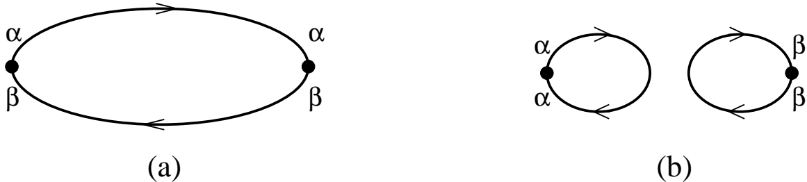
FIG. 1: Valence quark contractions in the scalar propagator G(x - y) , corresponding to Eq. (29). The solid dots represent the source \sigma . Only the valence quark lines are shown; completely disconnected contributions to (b) should be omitted.
