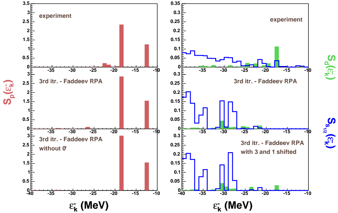
Figure 47: One-proton removal strength as a function of the hole sp energy \varepsilon_k^- = E_0^A - E_k^{A-1} for ^{16}\text{O} for angular momentum \ell = 1 (left) and \ell = 0, 2 (right). For the positive parity states, the solid bars correspond to results for d_{5/2} and d_{3/2} orbitals, while the thick lines refer to s_{1/2} . The top panels show the experimental values taken from [198]. The middle panels give the theoretical results for the self-consistent spectral function. The bottom panels show the results obtained by repeating the 3 rd iteration with a modified ph-DRPA spectrum, in which the lowest eigenstates have been either removed or shifted to the corresponding experimental values.
