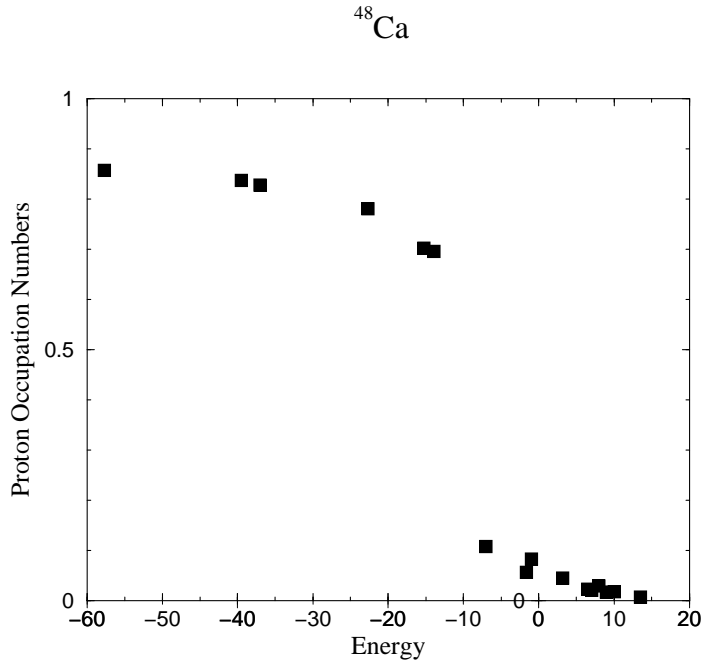
Figure 39: Proton shell occupation probabilities deduced from a comparison of the present calculation and the (e,e'p) data [201]. The figure displays the calculated values with the ppTDA correlations in the self-energy, multiplied by a factor 0.9 to simulate the effect of short-range correlations.
