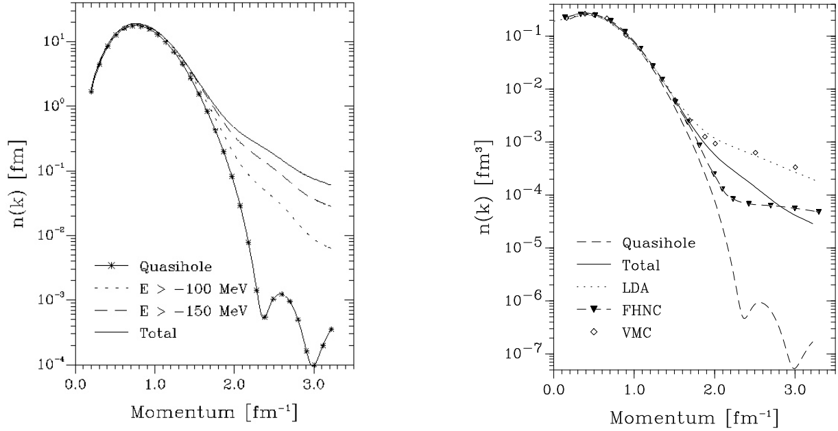
Figure 44: The total momentum distribution of ^{16}\text{O} . The left panel also displays the quasihole contribution and the results obtained with various energy cut-offs in the integration of the spectral functions. The right panel compares the momentum distribution obtained with the Green's function (total) with that of other approaches: local density approximation (LDA) [179], Fermi hypernetted chain (FHNC) [210] and Variational Monte Carlo (VMC) [173]. It should be noted that different normalizations were used for the presentation of these panels.
